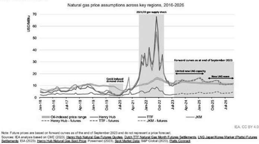
Forward curves suggest that natural gas prices will remain above their historical averages in the medium term
