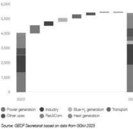
Natural gas demand outlook by sector, 2022-2050 (bcm)
